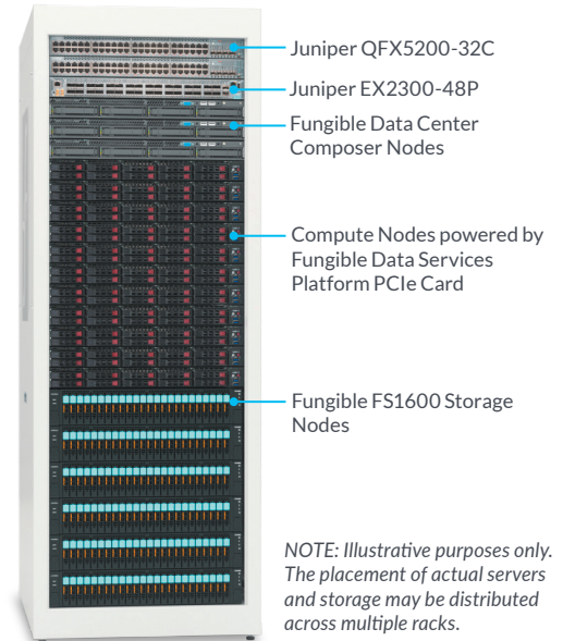
Figure 3: Fungible Data Center
